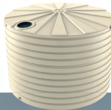
30000L (6600gal) T6500 ROUND QLD NSW VIC SA Inlet (H) 2.68m (8'9") Diameter 3.92m (12'10") Total (H) 2.87m (9'5")
