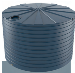
15000L (3300gal) TXD3300 ROUND QLD NSW VIC Inlet (H) 2.20m (7'3") Diameter 3.08m (10'1") Total (H) 2.48m (8'2")
