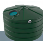
2400L (530gal) TS540 SQUAT QLD NSW Inlet (H) 1.06m (3'6") Diameter 1.81m (5'11") Total (H) 1.20m (3'11")
