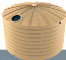
22500L (5000gal) TXD5000 SQUAT QLD NSW VIC SA Inlet (H) 2.20m (7'3") Diameter 3.78m (12'5") Total (H) 2.56m (8'5")
