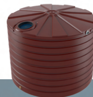
15000L (3300gal) T3300 ROUND SA Inlet (H) 2.20m (7'3") Diameter 3.05m (10'0") Total (H) 2.44m (8'0")
