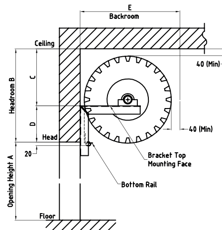
Elevation View
