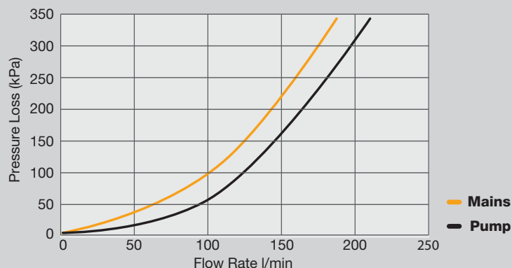
Pressure Loss Vs Flow Rate
