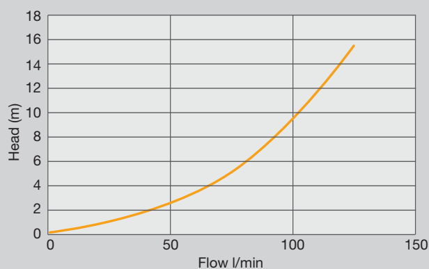
V-PC Pressure Loss
