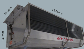
Cubic Evaporator 3 Fan Approx. weight 31kg
