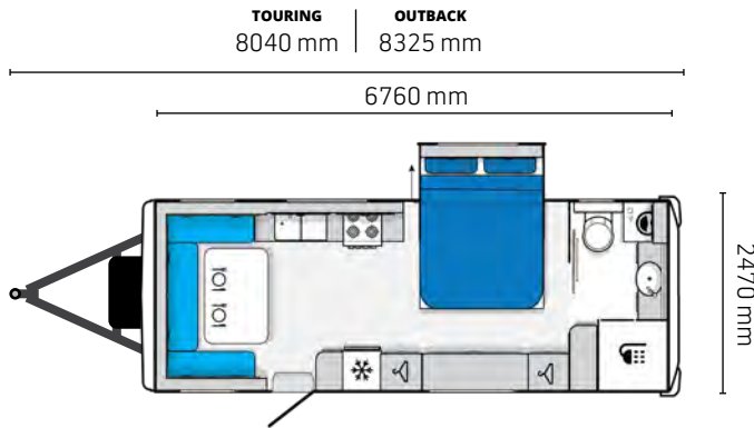
21 ft Club 21.63-3 Tandem Axle Caravan
