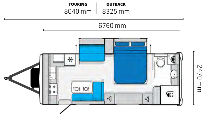
21 ft Dual Slide 21.65-4 Tandem Axle Caravan
