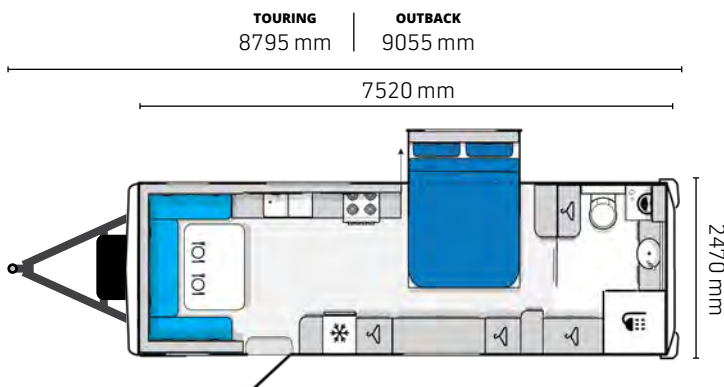
24 ft Club 24.75-2 Tandem Axle Caravan
