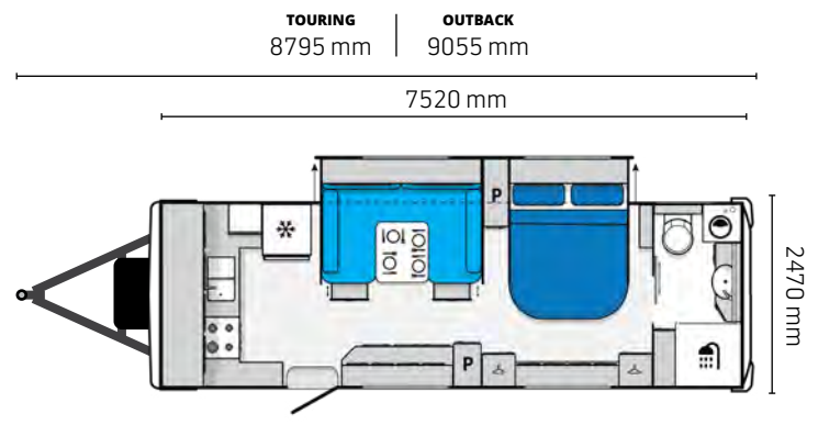
24 ft Dual Slide 24.75-4 Tandem Axle Caravan
