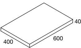
STANDARD PAVER
