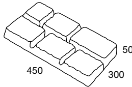
COBBLES
