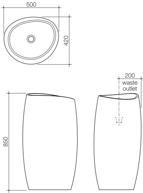
01 Muze Freestanding Basin - NTH EU8603A00W
