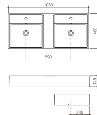
06 Teo 1050 Wall Basin – 2TH EU8035A25W
