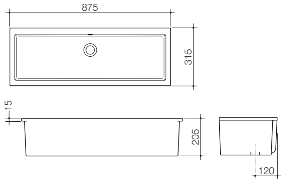
04 Quinn 875 Under Counter Basin - NTH EU8092A05W
