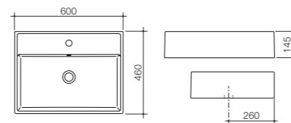
02 Teo 600 Wall Basin – NTH & 1TH EU8031B05W, EU8031B15W
