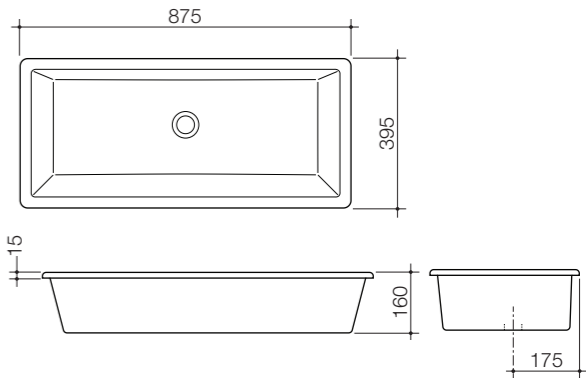
04 Quinn 875 Under Counter Basin - NTH EU8092A05W
