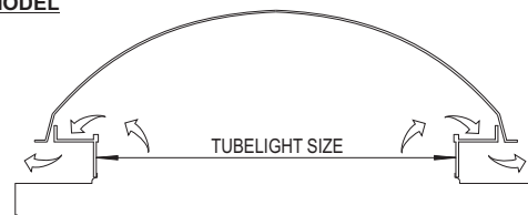
NON-VENTED MODEL
