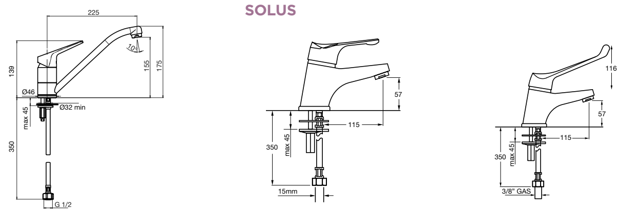
SOLUS MKII STANDARD SINK MIXER
