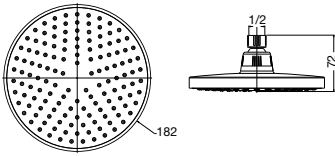
DOMAINE ROUND OVERHEAD SHOWER 180MM
