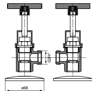
SOLUS WASHING MACHINE STOPS
