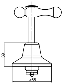
BRISTOL LEVER WALL TOP ASSEMBLY
