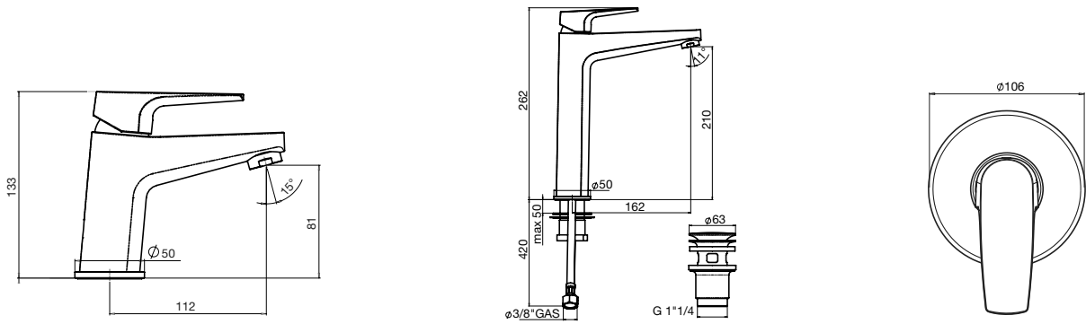
SOLUS MKII BASIN MIXER
