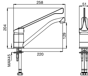
BRISTOL MKII SINK MIXER WITH EXTENDED LEVER
