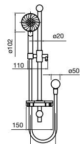
SOLUS MKII 1 OR 5 FUNCTION BRASS RAIL SHOWER
