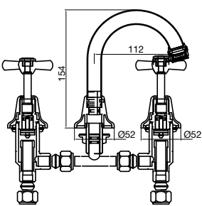
BRISTOL BASIN SET
