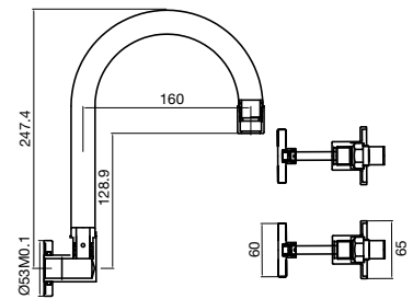
SOLUS WALL SINK SET
