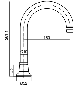
BRISTOL HOB OUTLET GOOSENECK 19MM
