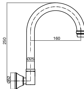
BRISTOL WALL OUTLET GOOSENECK
