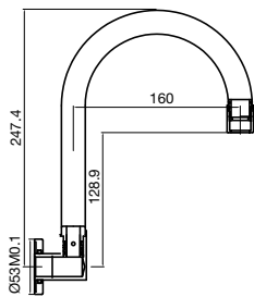
SOLUS WALL SINK OUTLET 200MM
