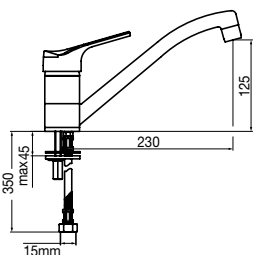
SOLUS SINK MIXER
