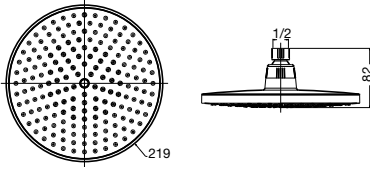
DOMAINE ROUND OVERHEAD SHOWER 220MM
