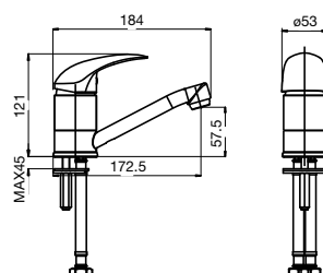
BRISTOL MKII SWIVEL BASIN MIXER
