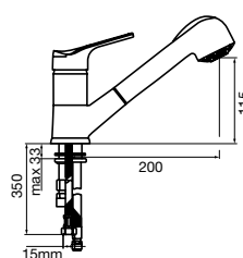
SOLUS SINK MIXER WITH PULL-OUT
