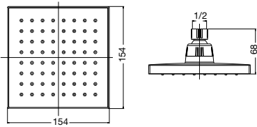
DOMAINE SQUARE OVERHEAD SHOWER 150MM
