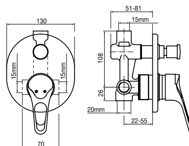
SOLUS SHOWER/BATH MIXER WITH DIVERTER
