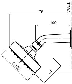
SOLUS MKII 1 OR 5 FUNCTION WALL SHOWER ON ARM
