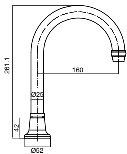
BRISTOL HOB OUTLET GOOSENECK 25MM
