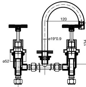
SOLUS BASIN SET
