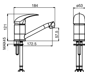
BRISTOL MKII BASIN MIXER
