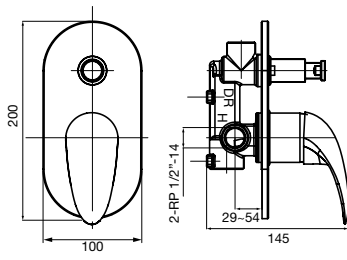
BRISTOL MKII SHOWER MIXER MIXER WITH DIVERTER
