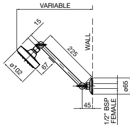
SOLUS MKII 1 OR 5 FUNCTION HI-RISE SHOWER
