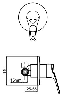
SOLUS SHOWER/BATH MIXER
