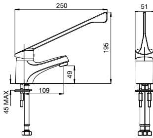
BRISTOL MKII BASIN MIXER WITH EXTENDED LEVER
