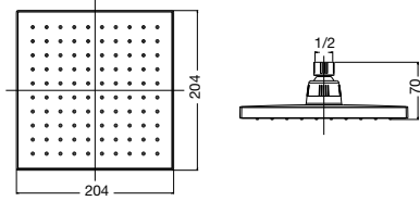
DOMAINE SQUARE OVERHEAD SHOWER 200MM
