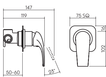
Wall Basin / Bath Mixer 6540.045A
