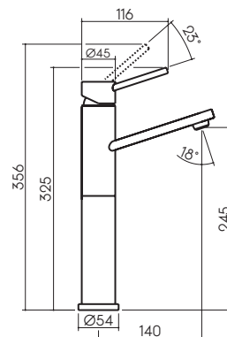
Tower Basin Mixer 6902.045A
