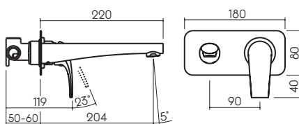
Wall Basin / Bath Mixer 6540.045A
