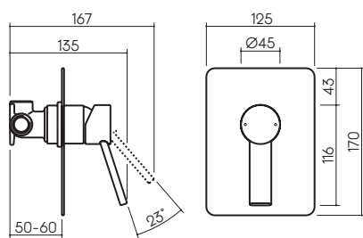
Wall Basin / Bath Mixer 6906.045A
