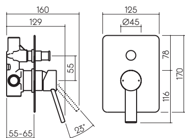
Bath / Shower Mixer w/ Diverter 6904.04
