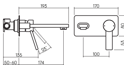
Wall Basin / Bath Mixer 6906.045A
