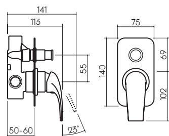
Bath / Shower Mixer w/ Diverter 6502.04
