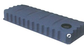
1000 Litre Underdeck 1200mm(w) x 3000mm(l) x 395mm(h) Tank comes with 1x1" BSP Brass Fitting + Inlet Strainer & 90mm Overflow Fitting (Underdeck tanks available in Black Only)
