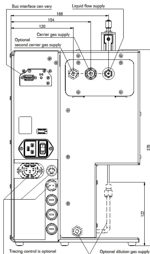
Rear view
