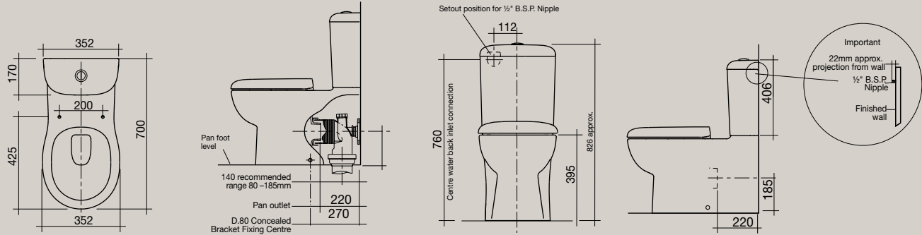
Pearl Back To Wall Toilet Suite An optional offset connector is available for set out of 186-220mm.
