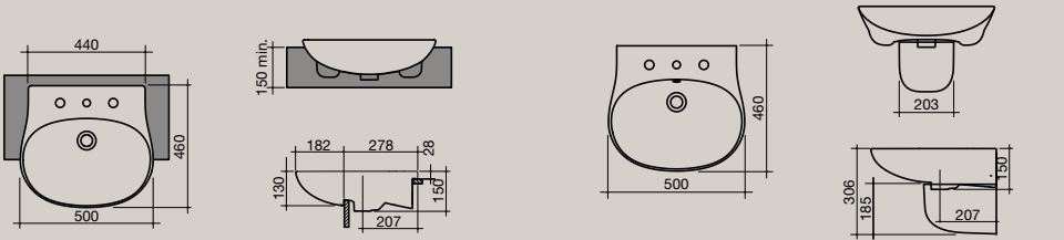
Pearl 500 Semi Recessed Basin
