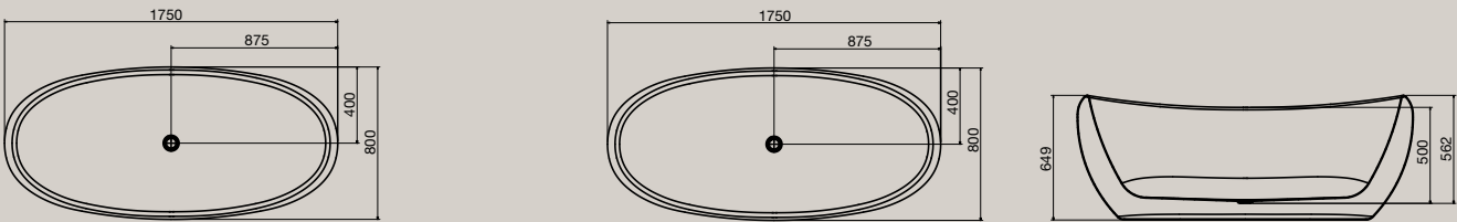
Pearl 1750 Island Bath
