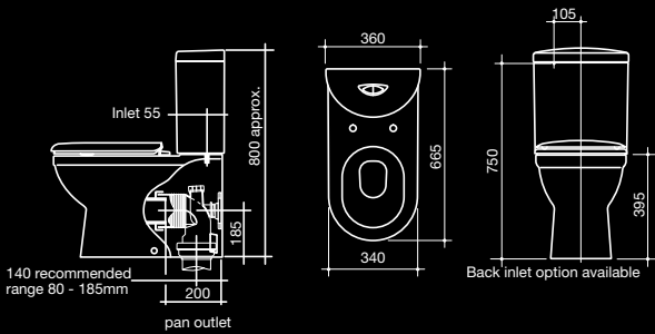
Milan Back to Wall Toilet Suite
