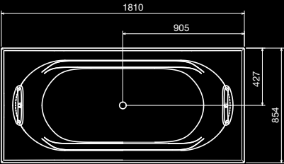
Milan 1800 Rectangular Bath
