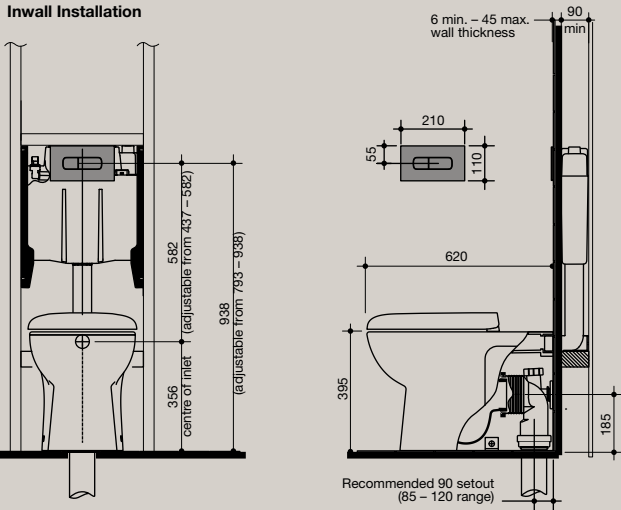
Pearl Wall Faced Invisi Toilet Suite
