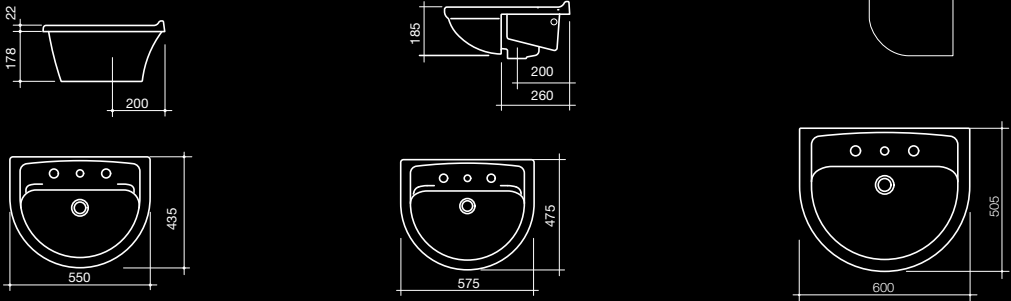
Milan 550 Vanity Basin
