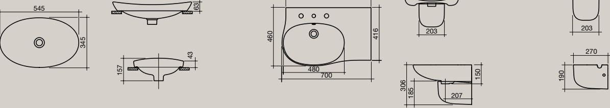
Pearl 550 Inset Basin
